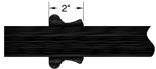
1-3/4" STANDARD PLANT-ON
