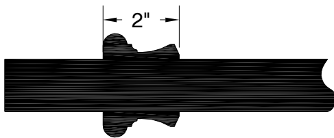
1-3/8" STANDARD PLANT-ON
