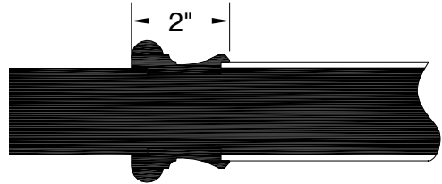
1-3/4" STANDARD MIRROR
