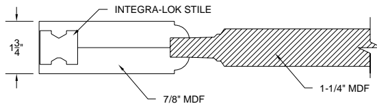
OVATION - 1-1/4" RAISED PANEL - 20 MIN. RATING
