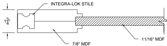
OVATION - 11/16" FLAT PANEL - 20 MIN. RATING
